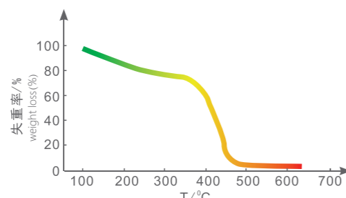
环氧树脂 (E-20) /AR 体系固化产物热重曲线 Thermogravimetry curve of curing product of epoxy resin E-20/AR system
