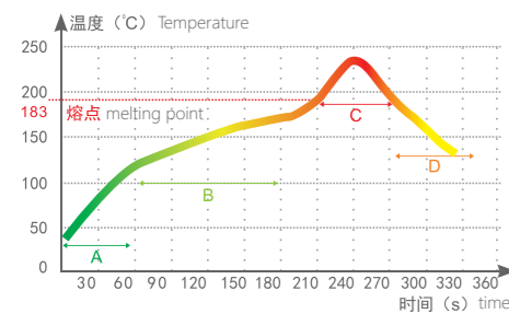
回流焊温度曲线图 Reflow soldering curve graph
